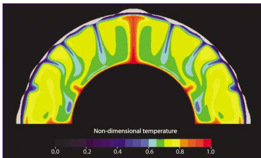
1: Numerical simulation of a deep mantle plume. The red, mushroom-like feature represents a hot upwelling from the core–mantle boundary. Blue, linear features are cold downwellings. (From Kiefer and Kellogg 1998.)
